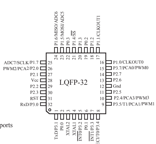
STC12C5620 series (without A/D Converter), LQFP-32
