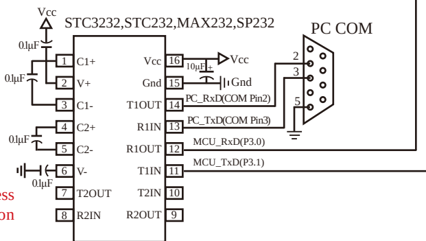
Circuit diagram for ISP of STC MCU , STC RS-232 Converter
