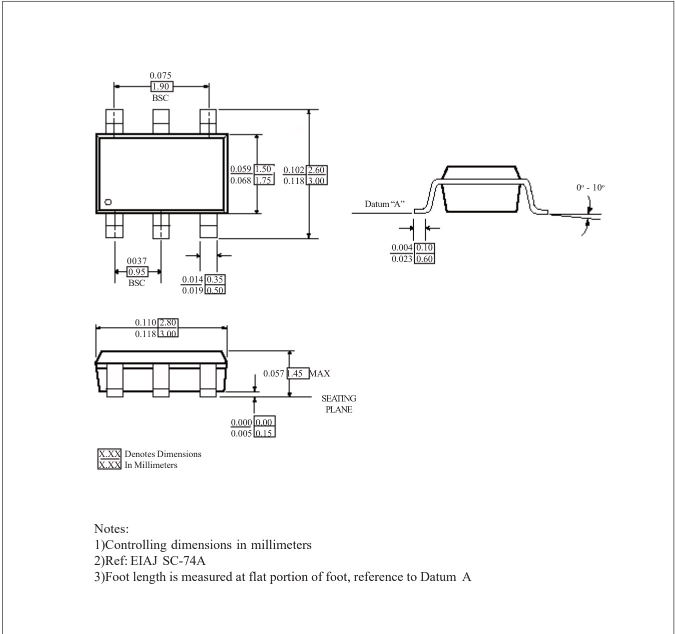
Figure 8. SOT23-6
