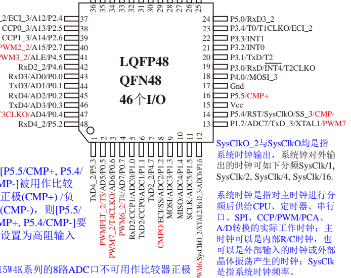
LQFP48 (9x9mm)
