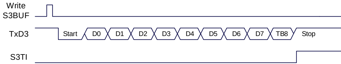
Transmitting data (Serial port 3 mode 1)
