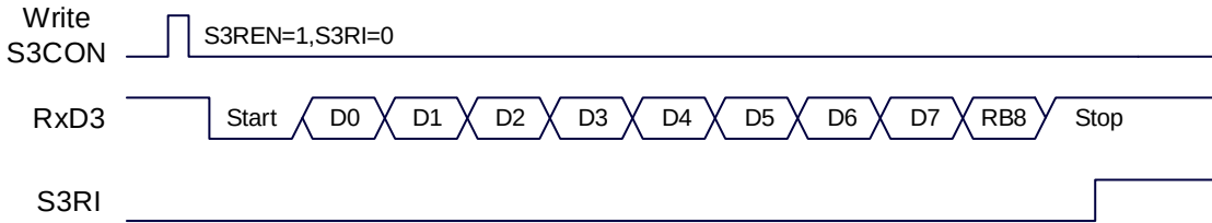
Receiving data (Serial port 1 mode 1)
